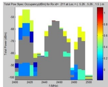
Spectrum Occupancy
